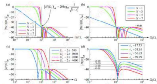
Figure 8.10 Dependence of the inverse Chebyshev filter on parameters N , \Omega_c , and \epsilon_p .
