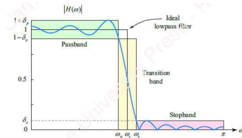
Figure 7.2 Specification of filter characteristics
