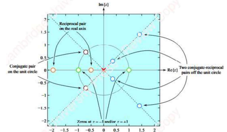
Figure 4.15 Position of zeros for linear-phase FIR systems
